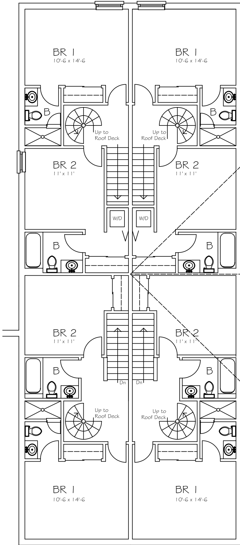
Scheme 3 Upper Level Scale: 1/8"=1'-0"
